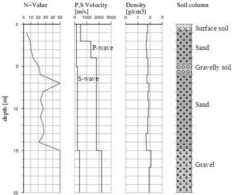
Fig. 1. Typical soil profile at HRS019 station, Japan (modified after www.K-net.bosai.go.jp )
