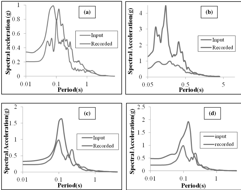
Fig. 3. Selected response spectra input and surface recorded used in the study (a) sand profile EHM006 with M_w 6.4 (b) clay profile FKS008 with M_w 9.0(c) gravel profile IWT023 with M_w 6.8 (d) mixed profile IWT009 with M_w 6.8
